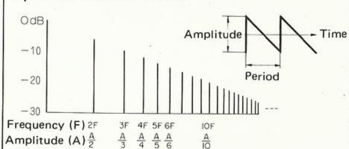
Spectrum of sawtooth wave
