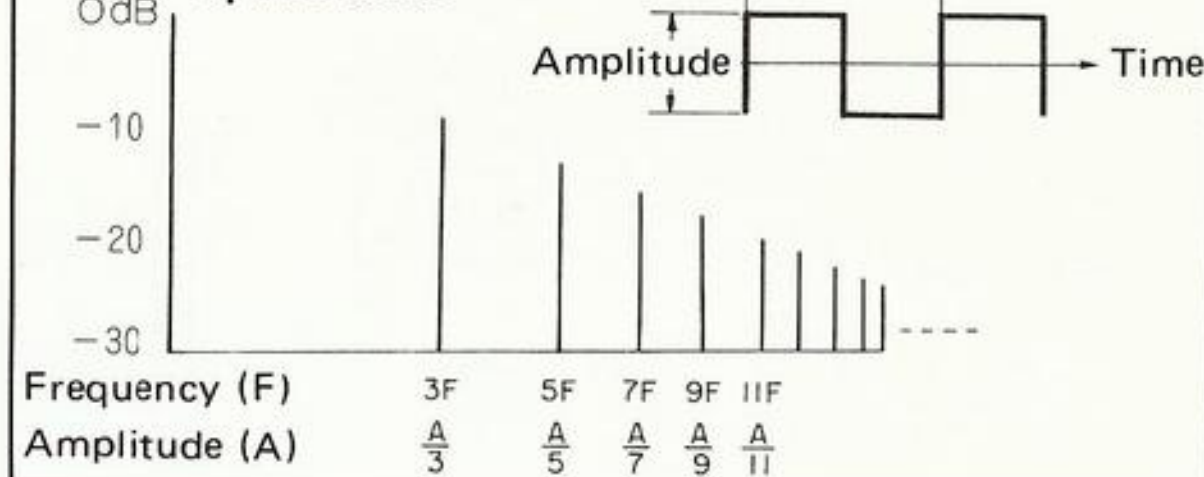
Spectrum of symmetrical square wave
